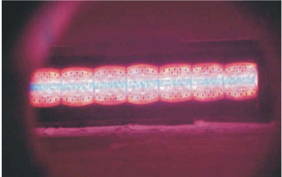
Good Burner as seen through entering end sight port
