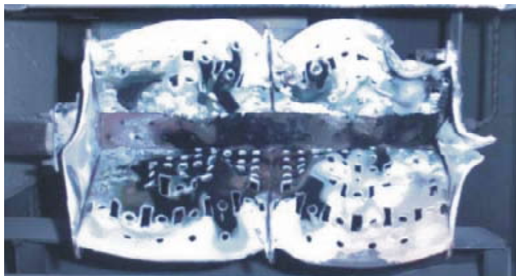
Acceptable mixing plate deformation
