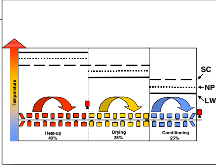
Innovation N° 3: Optimum zone length and special temperature profiles for each paper grade increase drying performance and reduce waste
