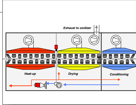
Dual Dry III process principle
